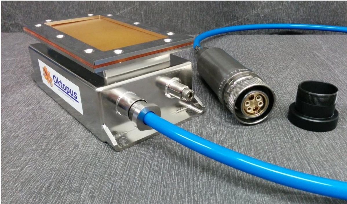
Figure 1: UKTB as a winch cable umbilical with Gisma BR40 connector
